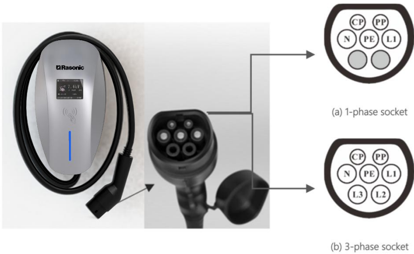
Fig. 3-2 Type 2 plug on RASONIC
